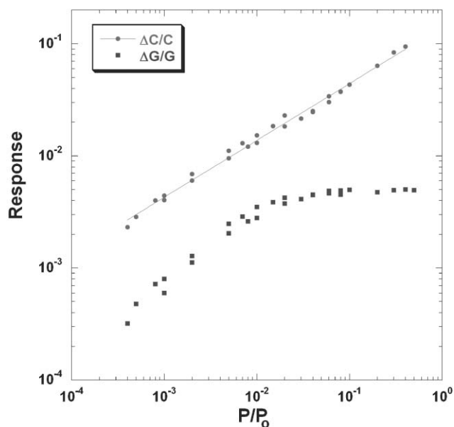
Fig. 9 Magnitude of the conductance and capacitance response as a function of acetone concentration. The conductance response saturates at about 0.01 P_0 , while the capacitance response continuously increases.
